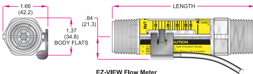
EZ-View Flow Meter (with Flow-Alert Reed Switch)
