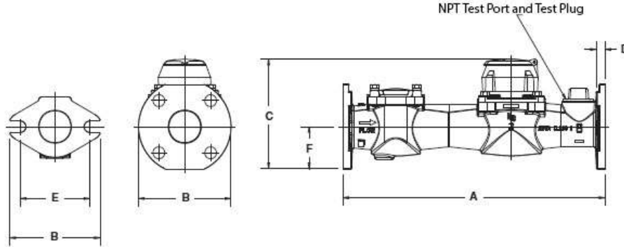
Figure 2: Physical dimensions
